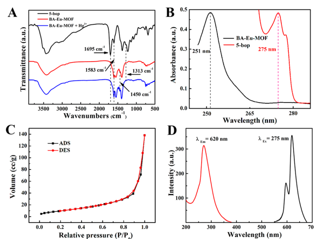
Figure 2. (A) FT-IR spectra of 5-bop (black), BA-Eu-MOF before (red) and after (blue) response to Hg 2+ . (B) UV-vis spectra of 5-bop (red) (0.01 mg/mL) and BA-Eu-MOF (black) (0.05 mg/mL). (C) Nitrogen adsorption (ADS) and desorption (DES) curves. (D) Emission (Em) spectra of BA-Eu-MOF with \lambda_{\text{Ex}} = 275 nm (black); excitation (Ex) spectra of BA-Eu-MOF with \lambda_{\text{Em}} = 620 nm (red).
