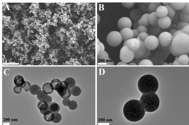
Figure 1. SEM images of BA-Eu-MOF with a ruler of 5 \mu m (A) and 200 nm (B). TEM images of BA-Eu-MOF with a ruler of 200 nm (C and D).
