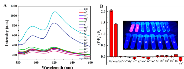
Figure 7. (A) Fluorescence spectra of BA-Eu-MOF toward various metal ions at the same concentrations (120 \mu\text{M} ). (B) (F - F_0)/F_0 of different metal ions; the inset shows the detection system of BA-Eu-MOF (0.3 mg/mL) in response to 120 \mu\text{M} concentrations of different metal ions under UV light at 365 nm (the white numbers correspond to the ions below from left to right).
